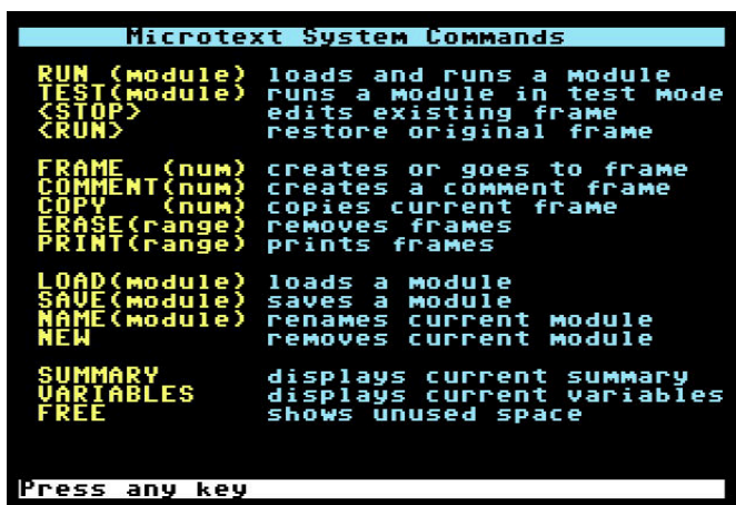
Fig.4 - Output of the HELP command
