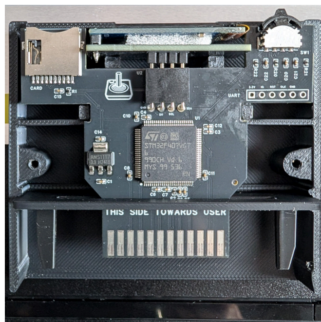
The printed circuit board with the ARM STM32F407VGT6 microcontroller in the center
