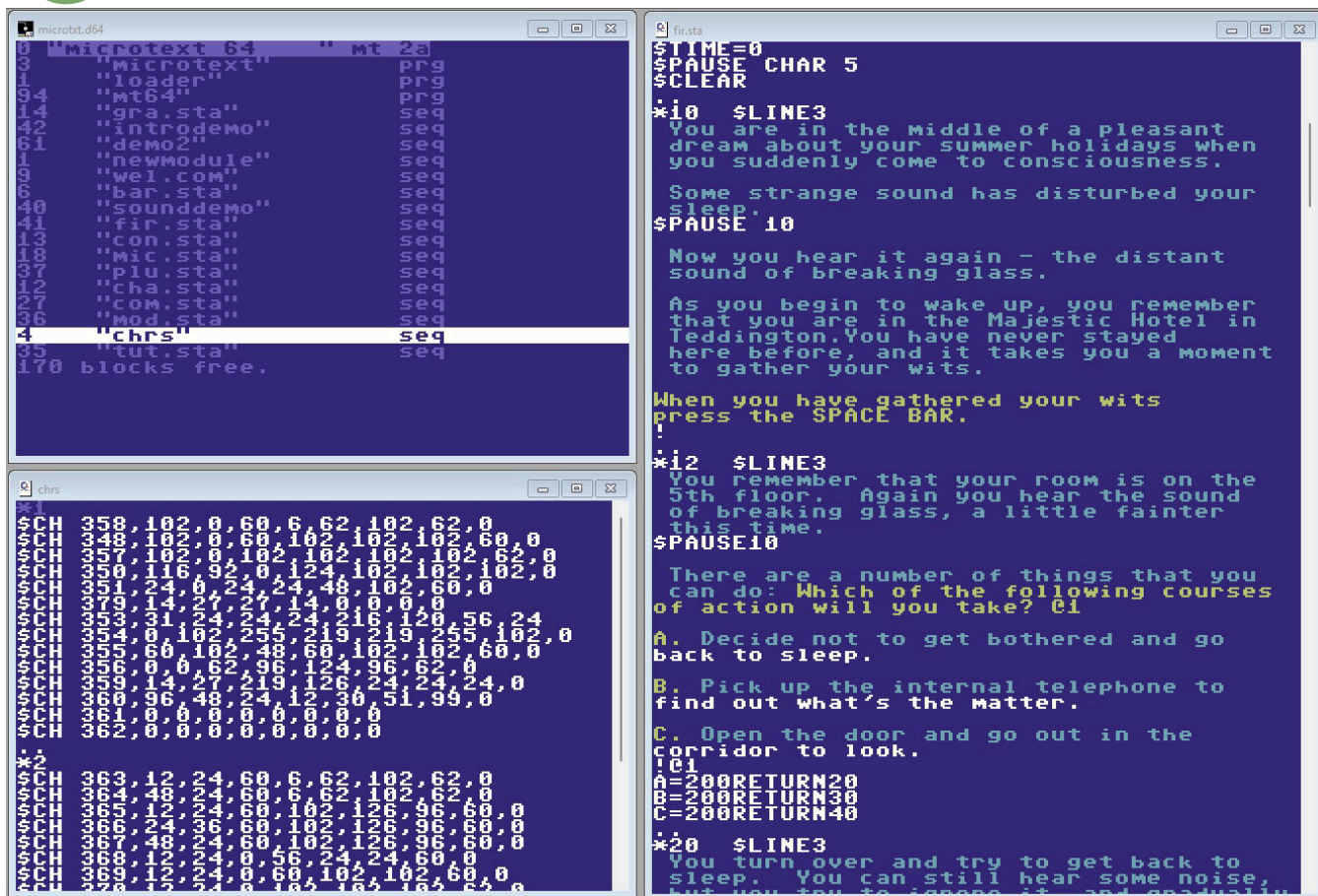
Fig.6 - Exploring the diskette with DIRMASTER
