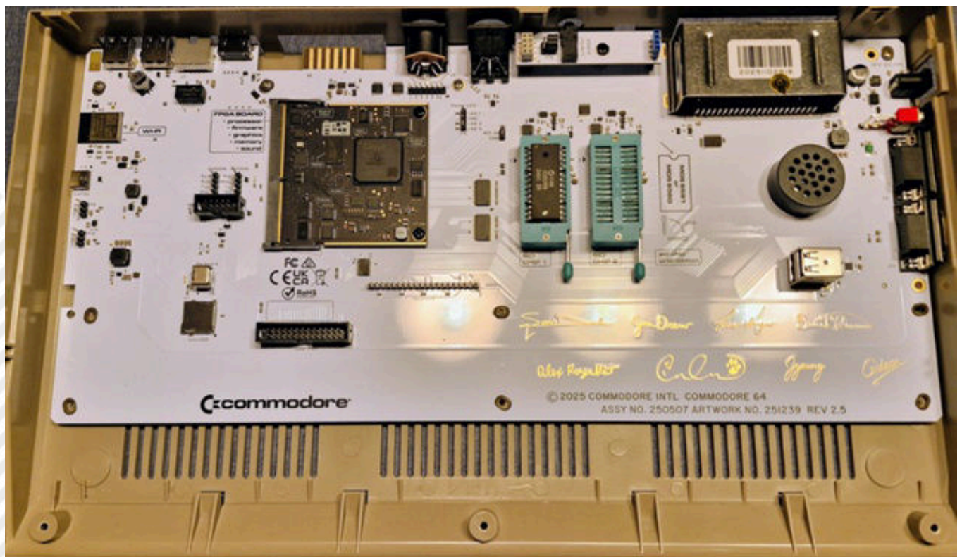
The C64 Ultimate PCB
